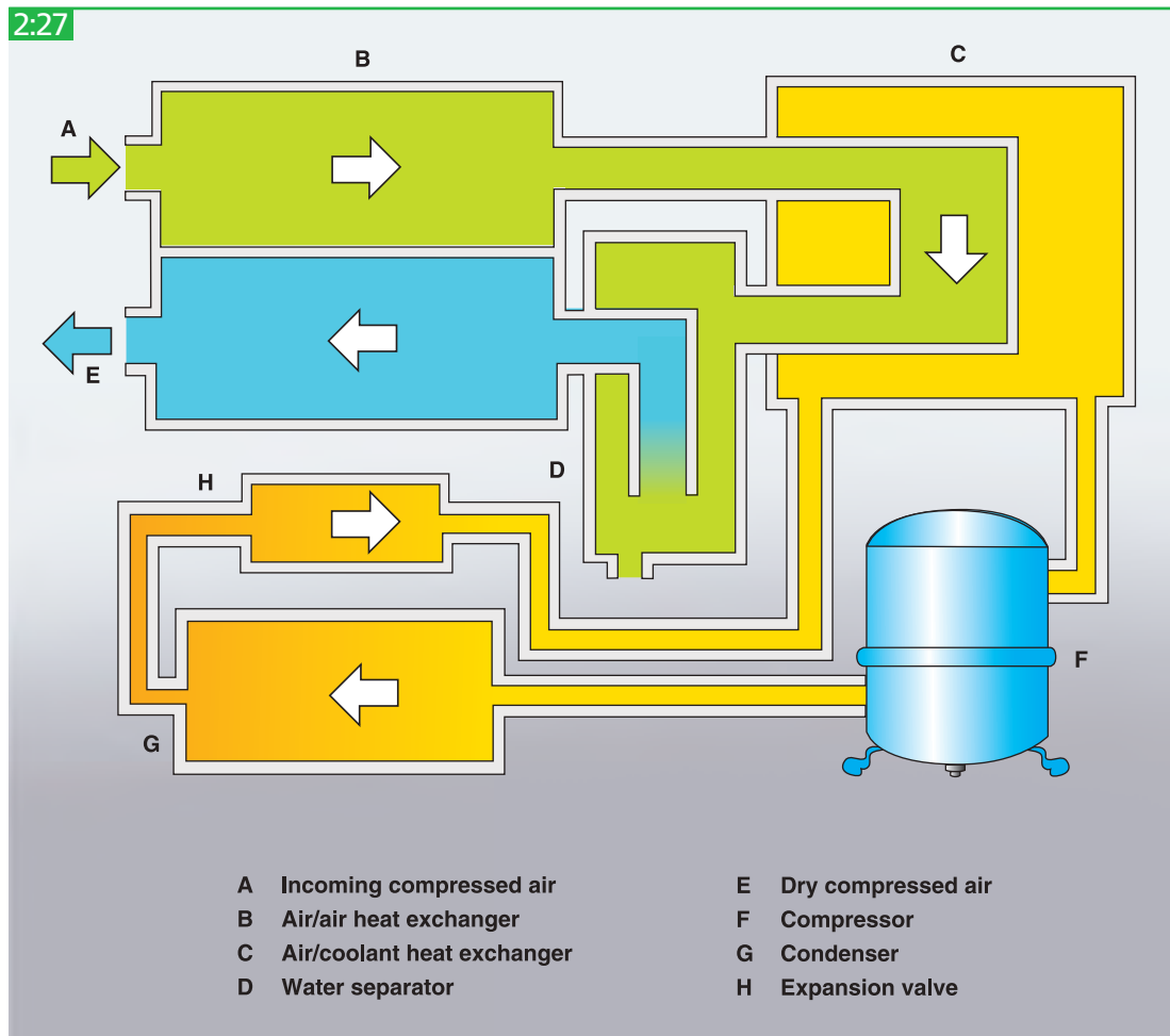
Operational principle of refrigerant drying.
